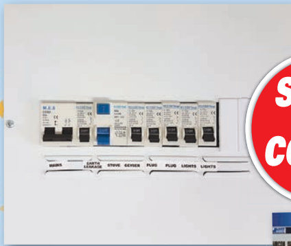
DISTRIBUTION BOARD
