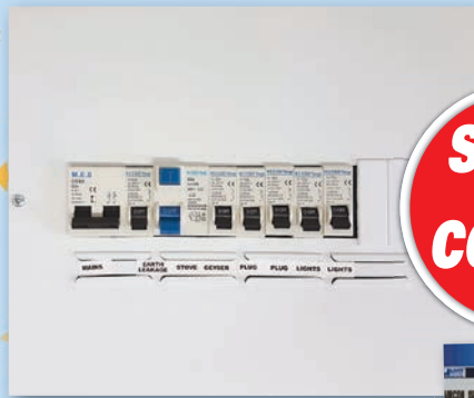
DISTRIBUTION BOARD
