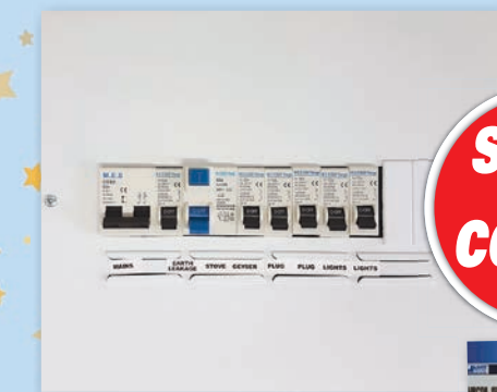
DISTRIBUTION BOARD
