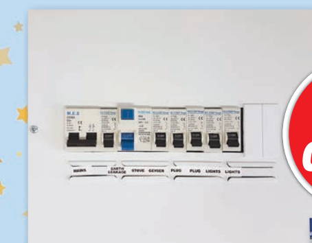
DISTRIBUTION BOARD
