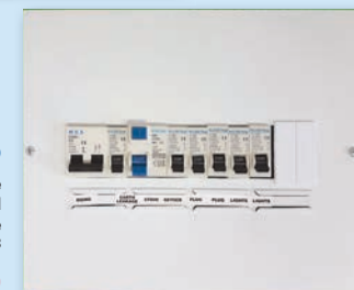
DISTRIBUTION BOARD
