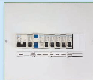
DISTRIBUTION BOARD
